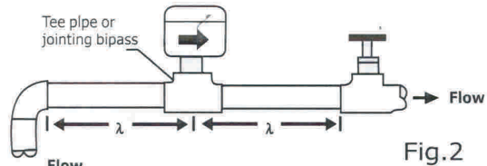
Size "λ" must be at least 5 times pipe from the nearest bend, valve or other throttling devices in pipe.
