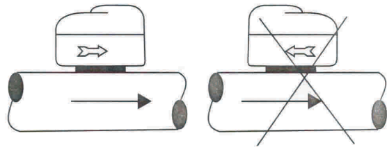
HF68 flow switch must be installed in the beeline pipe, which have at least 5 times pipe larger on both of the side (See Fig.2).
