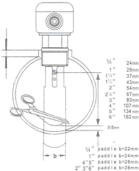
Fig.1 Adjust Flow Paddle
